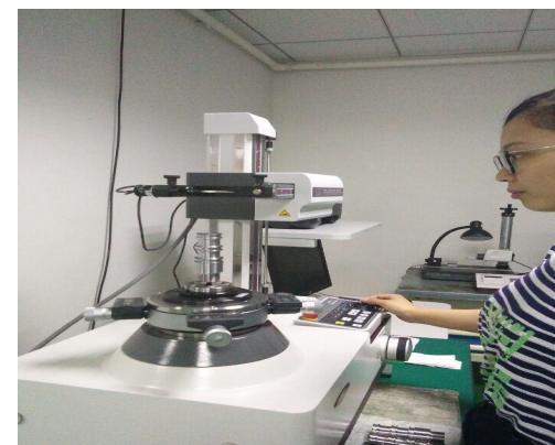
圆柱度仪 Cylindricity Tester
